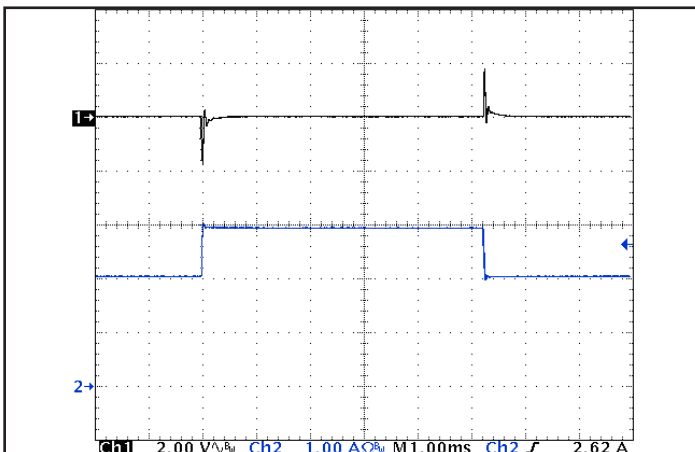
Figure 5: Output voltage response to step-change in load current (66% -100% -66% of I_{out(max)} ; dI/dt = 0.05 A/\mu s ). Load cap: 1 \mu F ceramic capacitor. Ch 1: V_{out} (2 V/div), Ch 2: I_{out} (1 A/div).
