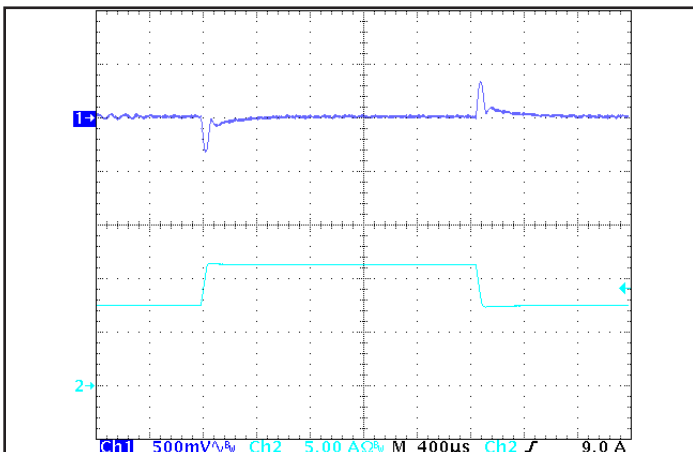
Figure 5: Output voltage response to step-change in load current (66% -100% -66% of I out(max) ; dI/dt = 0.1 A/µs). Load cap: 1 µF ceramic and 15 µF tantalum capacitors. Ch 1: V out (500 mV/div), Ch 2: I out (5 A/div).
