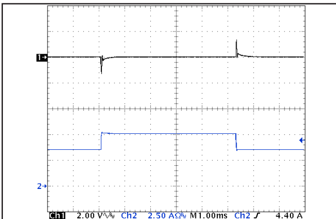
Figure 5: Output voltage response to step-change in load current (66% -100% -66% of I_{out(max)} ; dI/dt = 0.1 A/\mu s ). Load cap: 1 \mu F ceramic and 15 \mu F tantalum capacitors. Ch 1: V_{out} (2 V/div), Ch 2: I_{out} (2.5 A/div).
