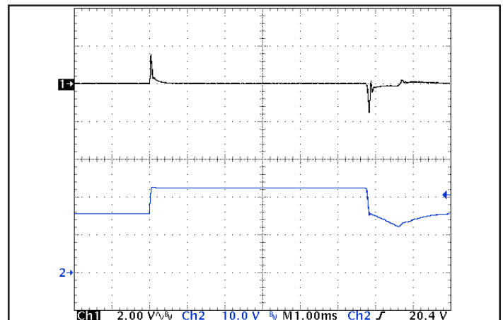
Figure 6: Output voltage response to step-change in input voltage (500 V/ms). Load cap: 100 \mu F , electrolytic output capacitance. Ch 1: V_{out} (2 V/div), Ch 2: V_{in} (10 V/div).
