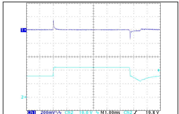
Figure 6: Output voltage response to step-change in input voltage (500 V/ms). Load cap: 100 \mu F , electrolytic output capacitance. Ch 1: V_{out} (200 mV/div), Ch 2: V_{in} (10 V/div).
