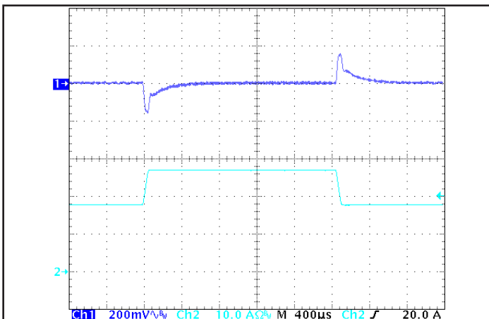
Figure 5: Output voltage response to step-change in load current (66% -100% -66% of I_{out(max)} ; dI/dt = 0.1 A/\mu s ). Load cap: 1 \mu F ceramic and 15 \mu F tantalum capacitors. Ch 1: V_{out} (200 mV/div), Ch 2: I_{out} (10 A/div).
