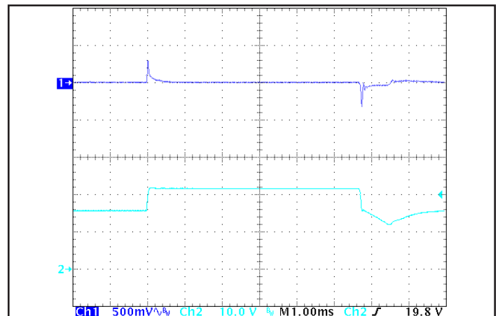
Figure 6: Output voltage response to step-change in input voltage (500 V/ms). Load cap: 100 µF, electrolytic output capacitance. Ch 1: V out (500 mV/div), Ch 2: V in (10 V/div).
